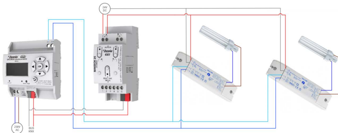
Figure 5. Wiring suggestion for the Standby function
