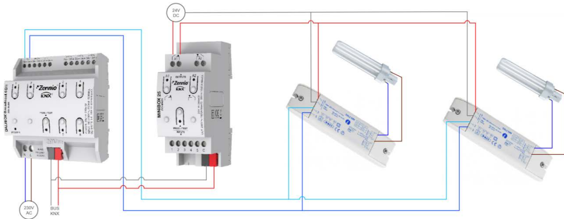
Figure 20. Standby Scheme
